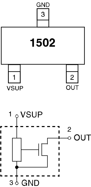
Fig. 4–5: Pin configuration
