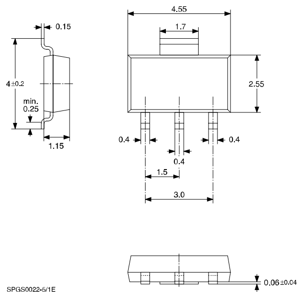
Figure 6: Plastic Small Outline Transistor Package ( SOT-89B ) Weight approx. 0.035 g Dimensions in mm
