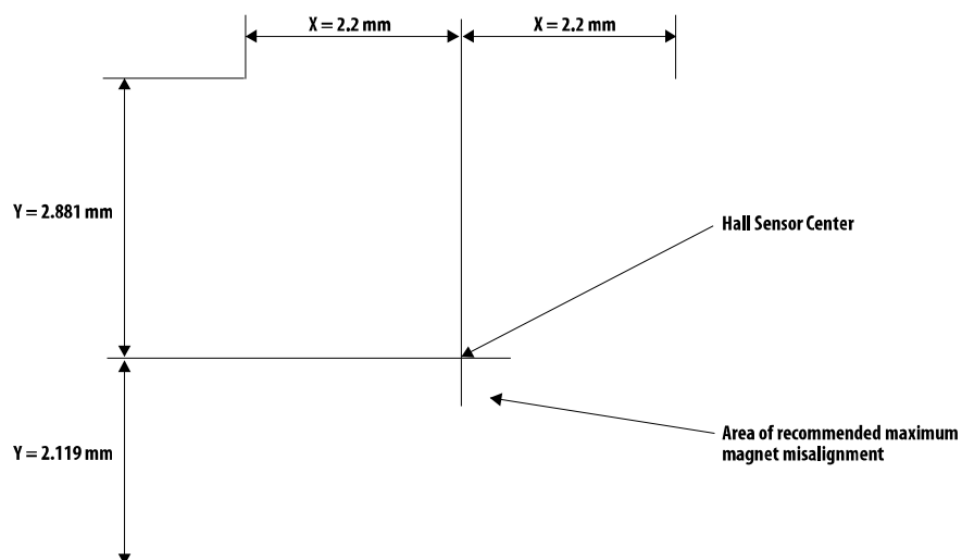
Figure 5. Magnet and IC Package Placement
