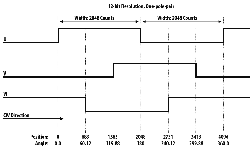
Figure 9. UVW commutation signals – 12-bit resolution, one-pole-pair
