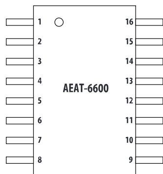
Figure 4. Pin Configuration TSSOP-16
