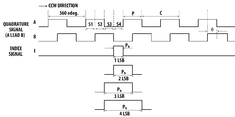
Figure 8. Incremental ABI signals
