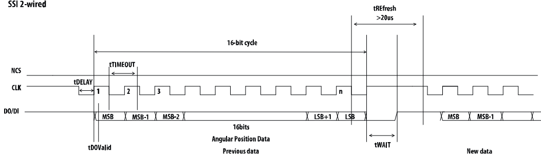
Figure 7. SSI Timing Diagram
