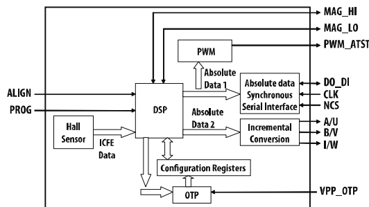
Figure 3. Polaris block diagram
