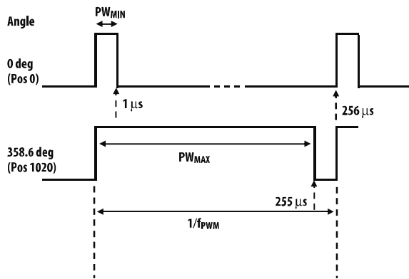
Figure 11. PWM signals – 12 bit resolution
