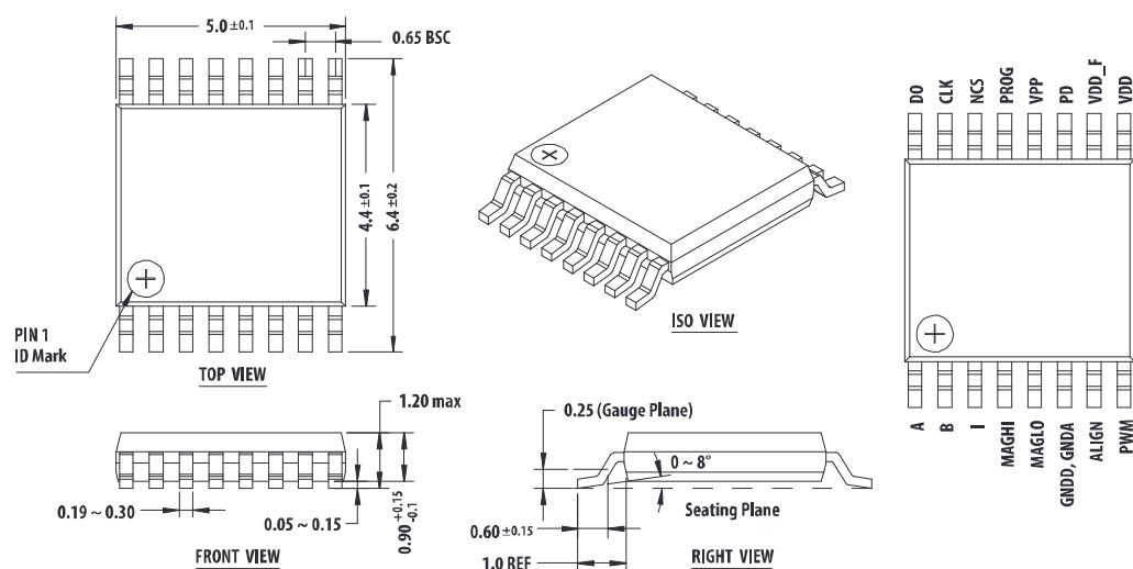
Figure 12. AEAT-6600, 16-Lead TSSOP dimensions
