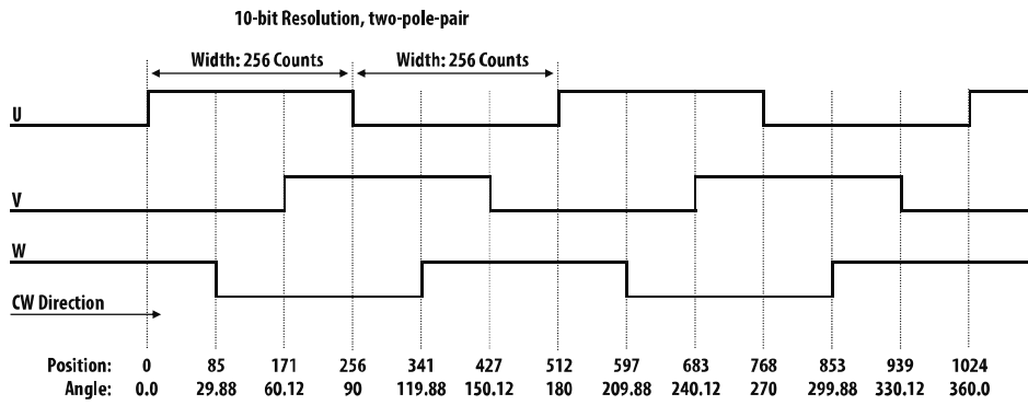
Figure 10. UVW commutation signals – 10-bit resolution, two-pole-pairs
