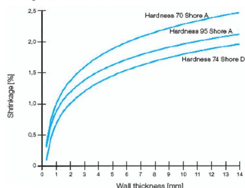
Shrinkage in relation to wall thickness
