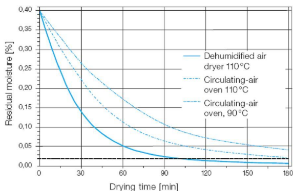
Drying diagram for Elastollan
