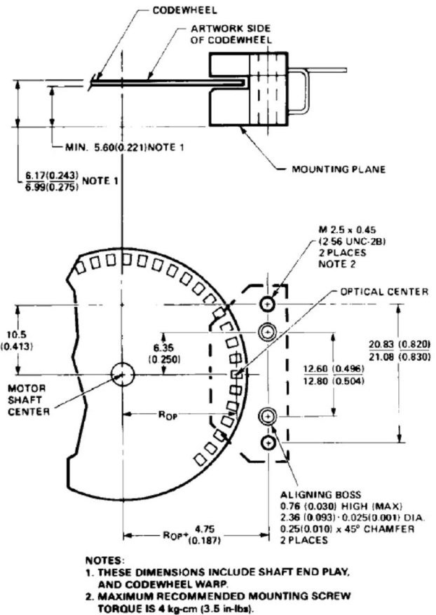
Figure 3. Mounting Plane Side B.
