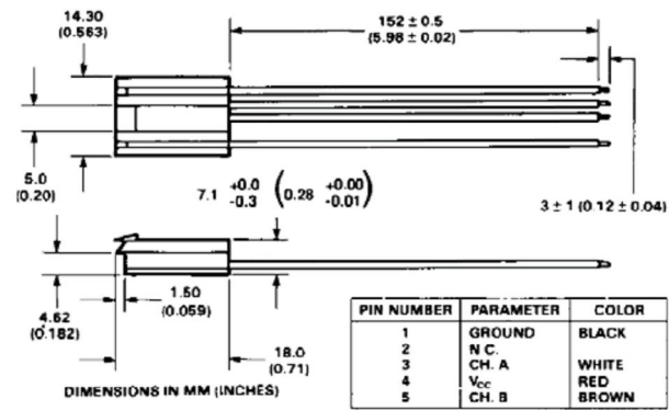
Figure 6. HEDS-8902 Connector.
