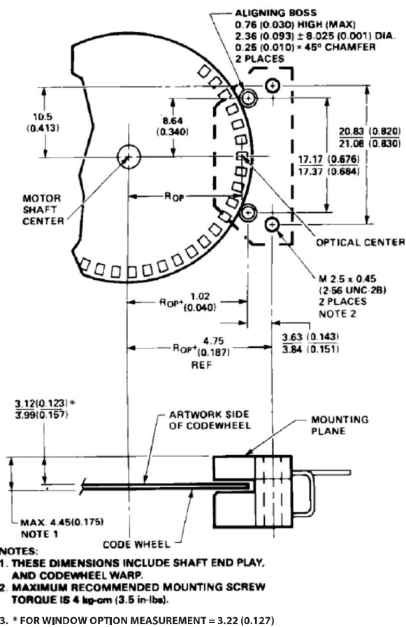
Figure 2. Mounting Plane Side A.
