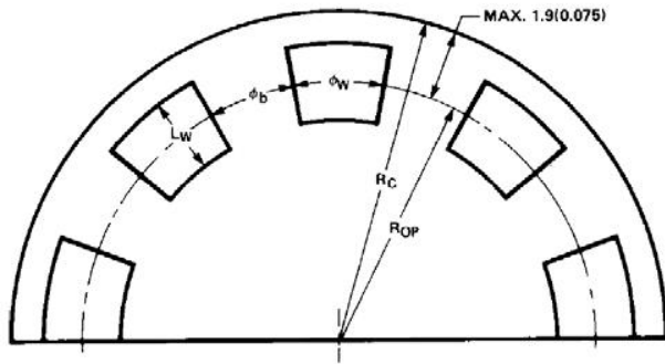
Figure 1. Codestrip Design
