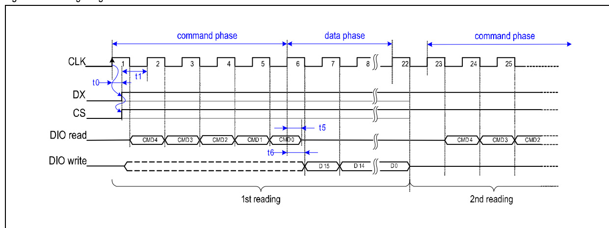
Figure 10. Timing Diagram in 2-wire SSI Continuous Readout
