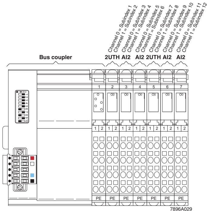
Figure 4-2 I/O station with analog input modules and thermocouple modules
