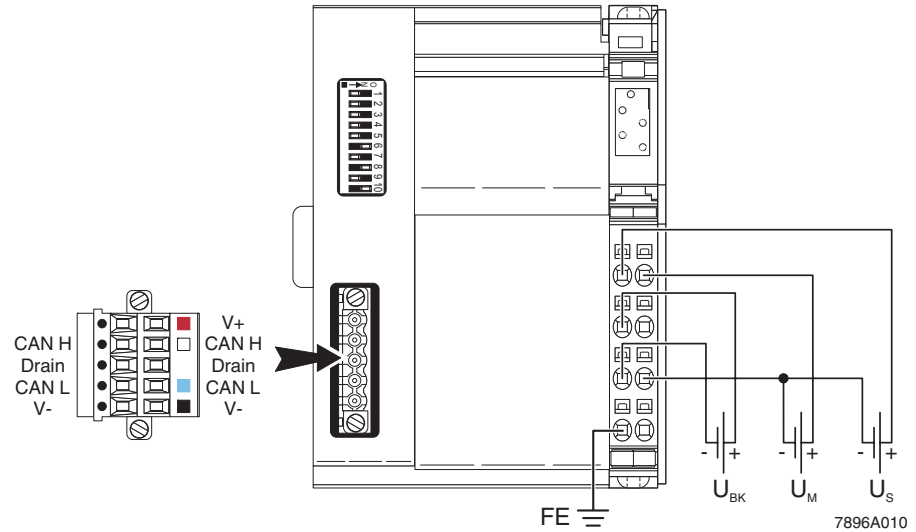
Figure 3-4 Typical bus coupler wiring
