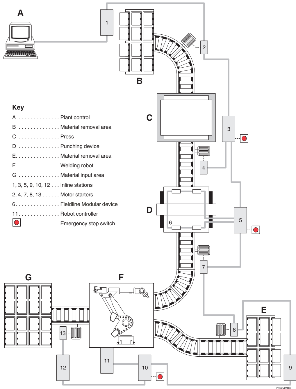
Figure A-3 Example plant layout controlled by a PC and using Inline
